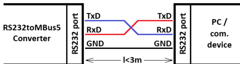
RS232 port connection between the converter and PC.
